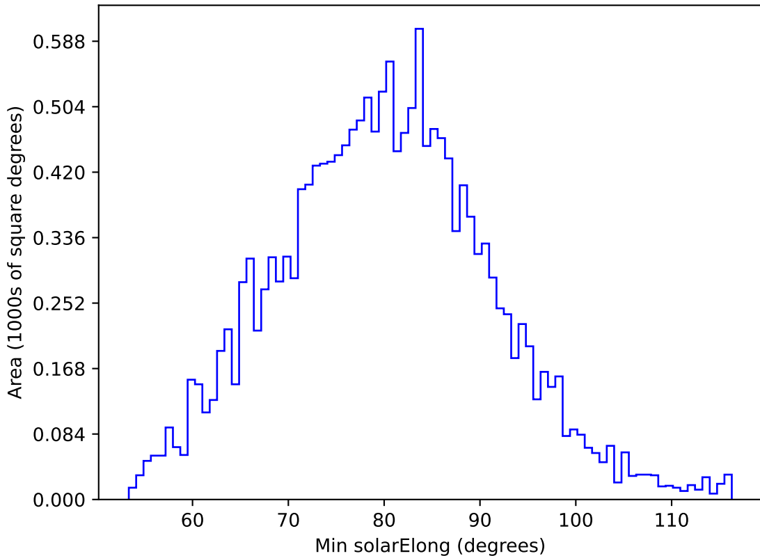
baseline_v2.0_10yrs WFD u band: Min solarElong
