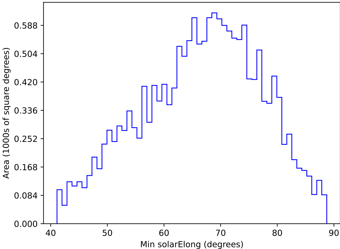
baseline_v2.0_10yrs WFD r band: Min solarElong
