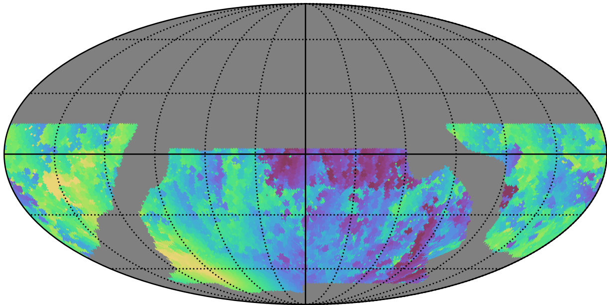
baseline_v2.0_10yrs WFD i band: Min solarElong
