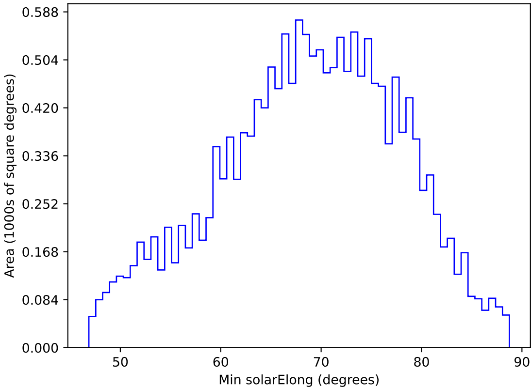
baseline_v2.0_10yrs WFD i band: Min solarElong
