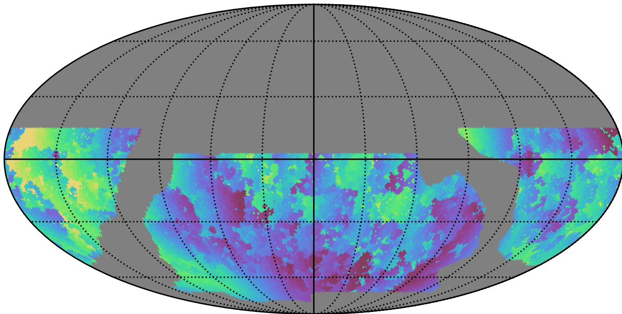
baseline_v2.0_10yrs WFD g band: Min solarElong
