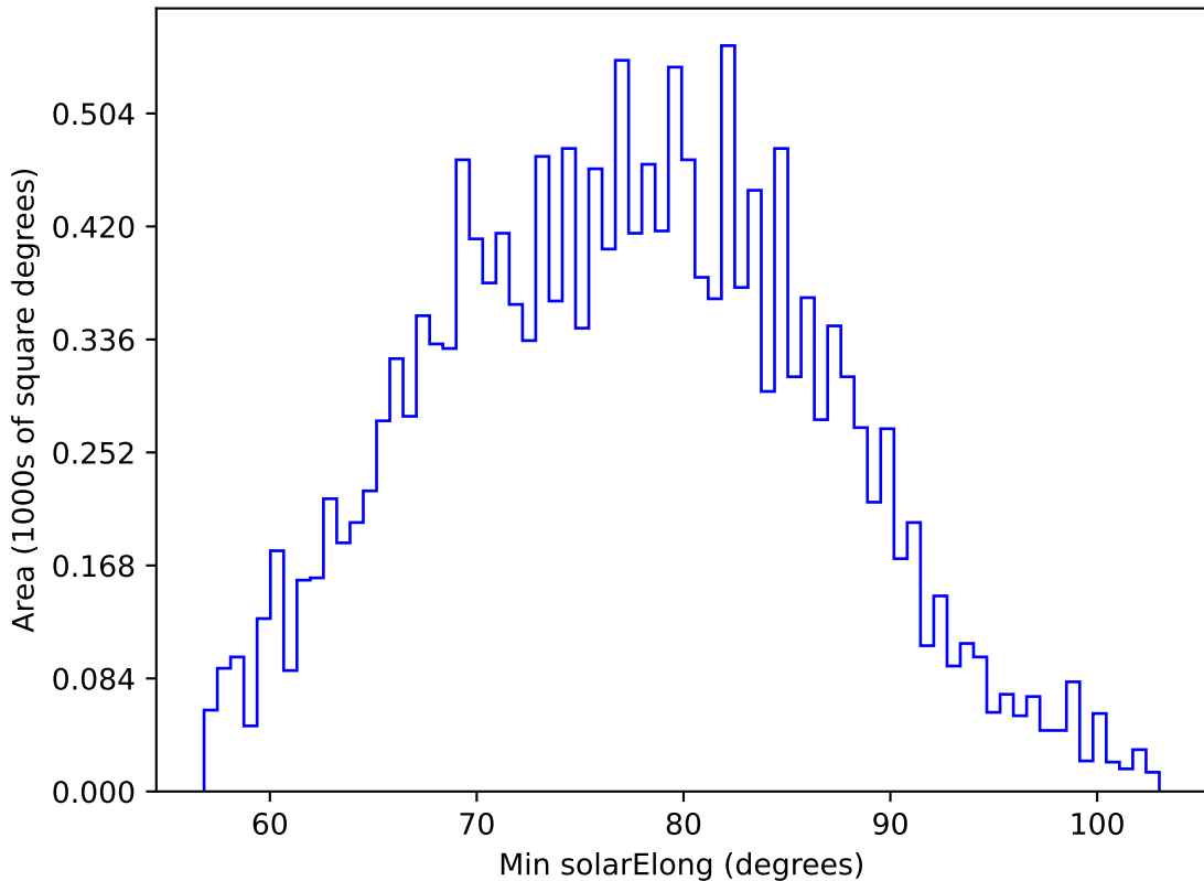
baseline_v2.0_10yrs WFD g band: Min solarElong
