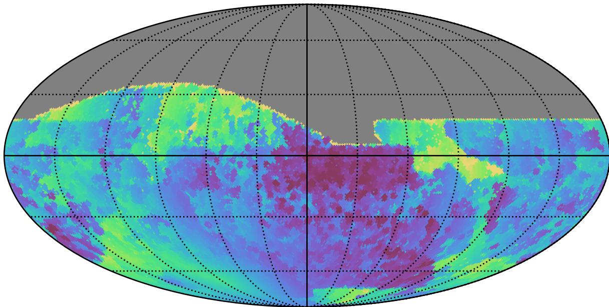
baseline_v2.0_10yrs All sky r band: Min solarElong
