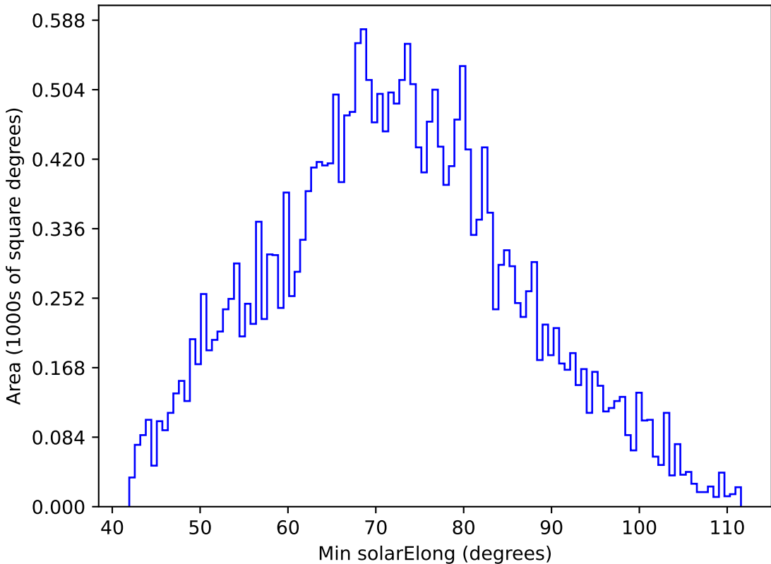
baseline_v2.0_10yrs All sky r band: Min solarElong
