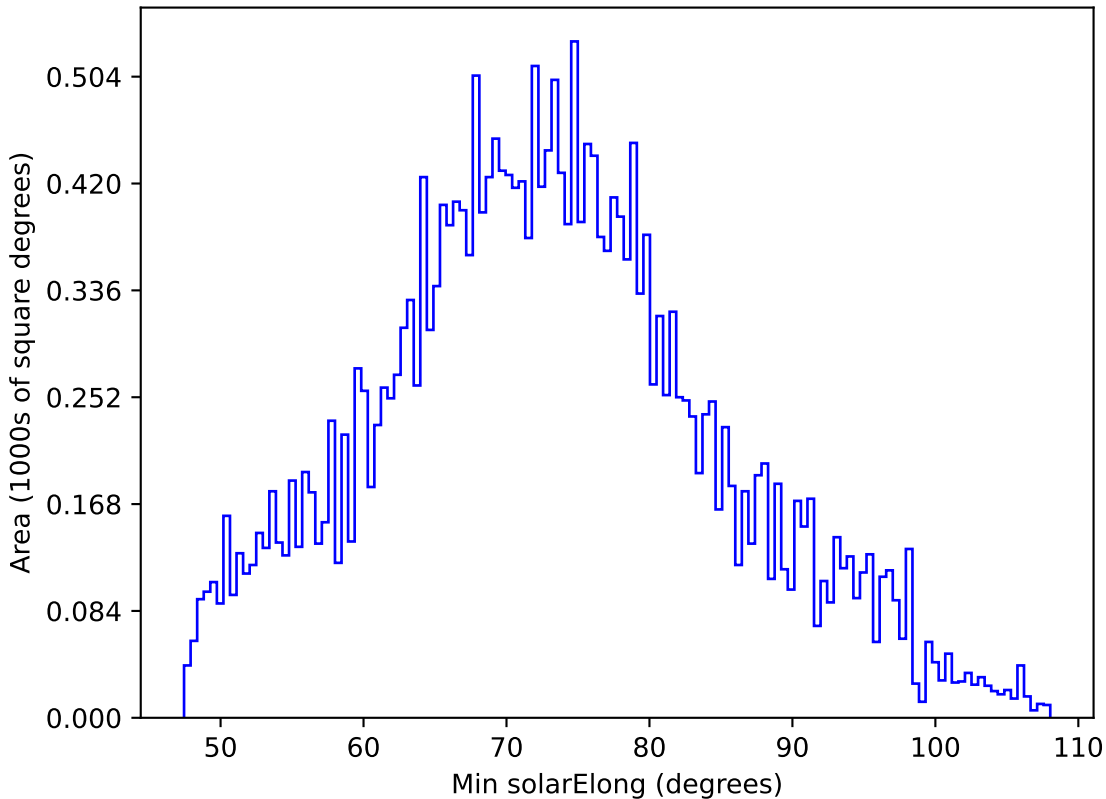
baseline_v2.0_10yrs All sky i band: Min solarElong
