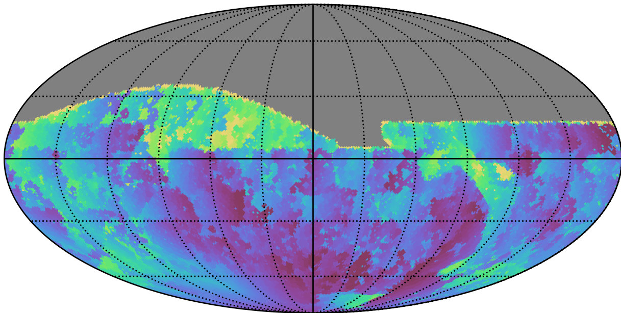
baseline_v2.0_10yrs All sky g band: Min solarElong
