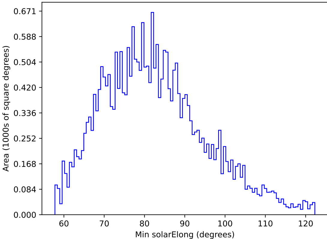
baseline_v2.0_10yrs All sky g band: Min solarElong
