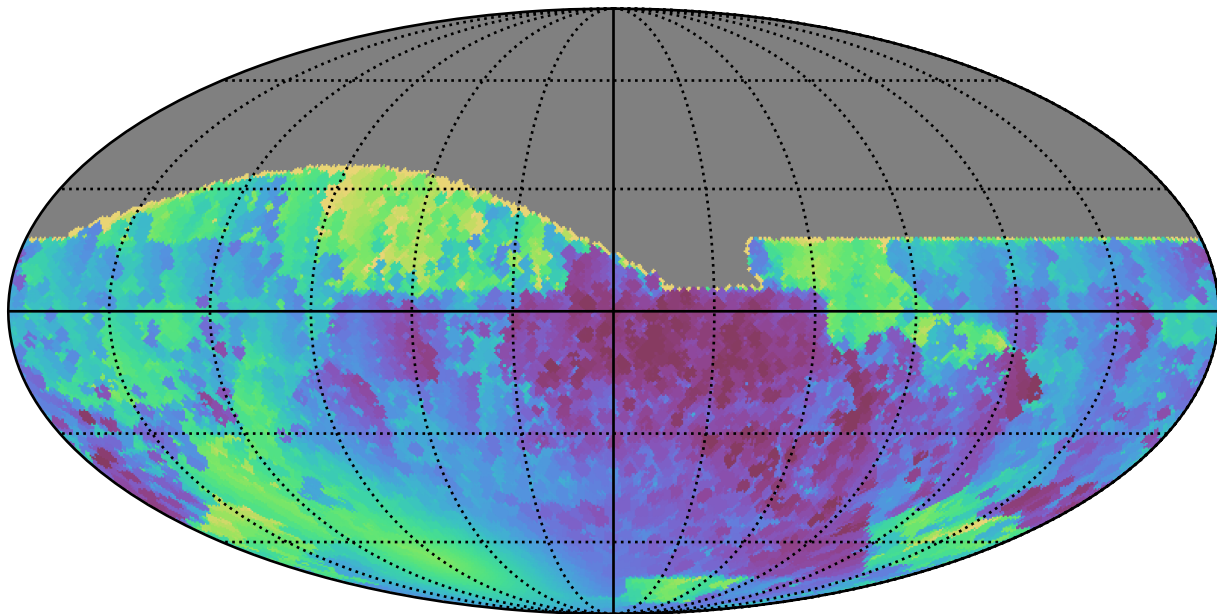
baseline_v2.0_10yrs All sky all bands: Min solarElong
