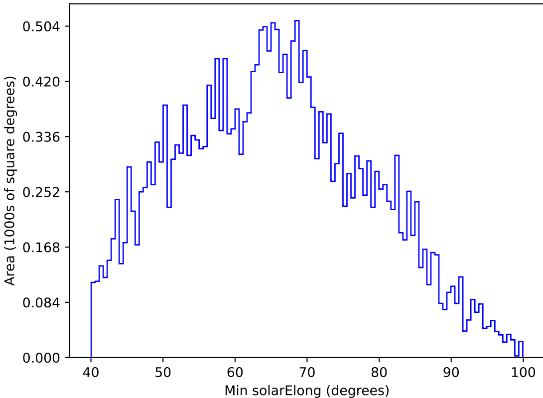
baseline_v2.0_10yrs All sky all bands: Min solarElong
