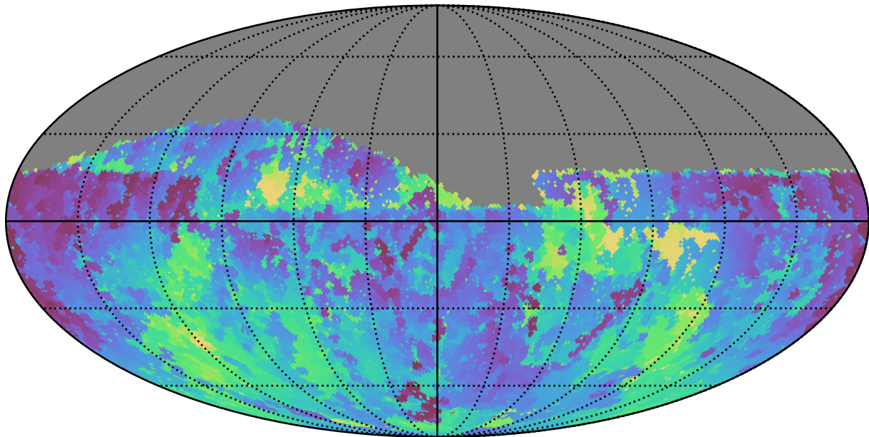
baseline_v2.0_10yrs Yr 1 z band: Min skyBrightness
