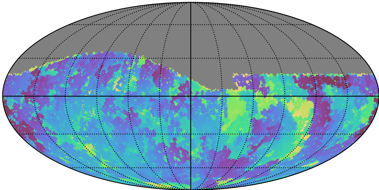
baseline_v2.0_10yrs Yr 1 i band: Min skyBrightness
