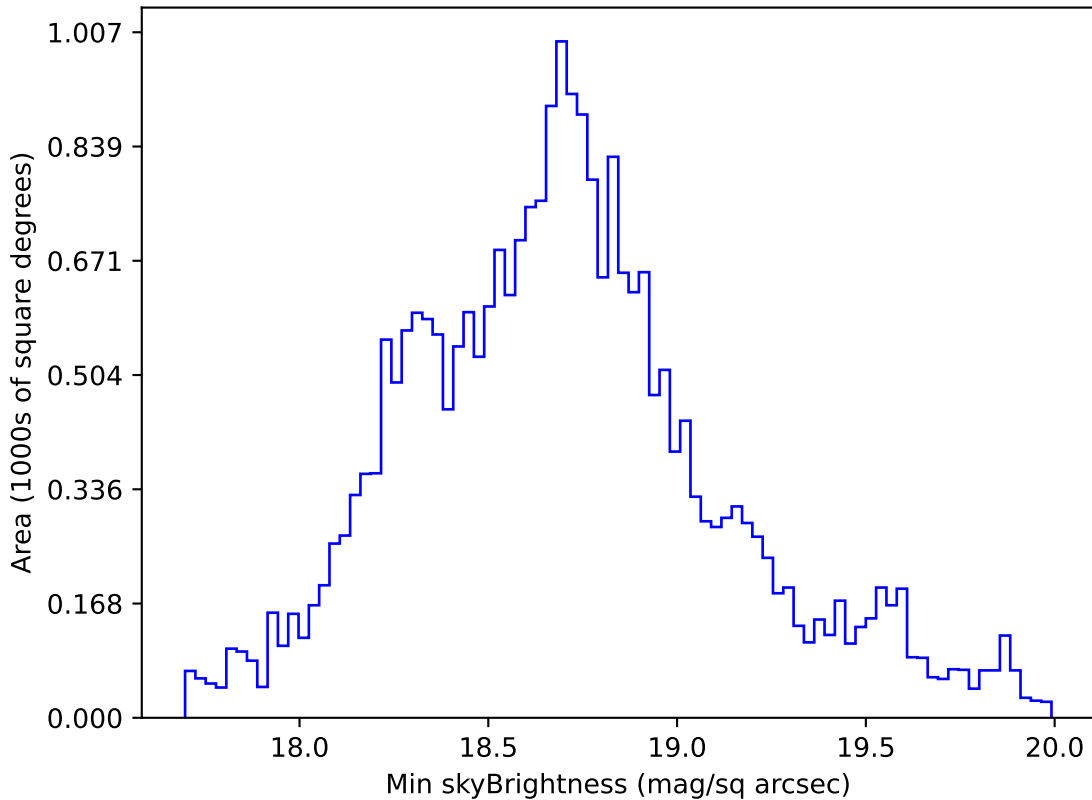
baseline_v2.0_10yrs Yr 1 i band: Min skyBrightness
