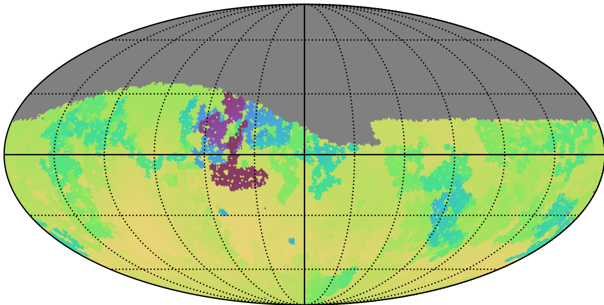
baseline_v2.0_10yrs Yr 1 g band: Min skyBrightness
