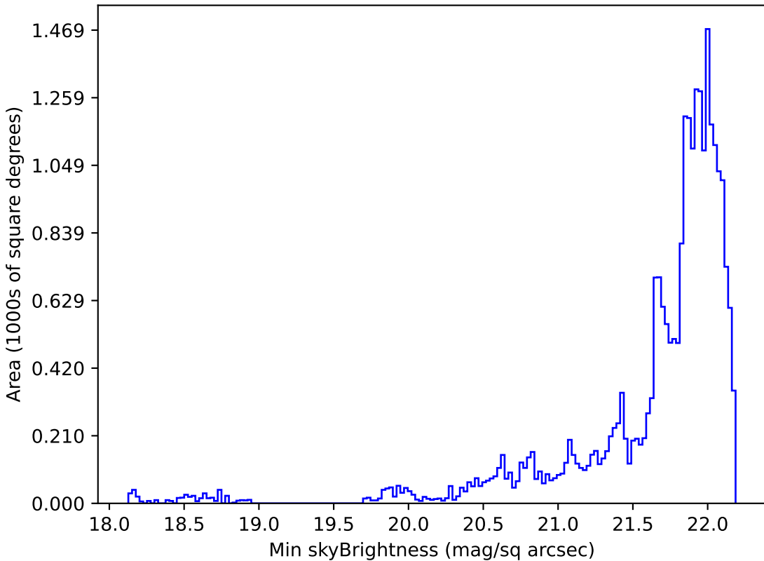
baseline_v2.0_10yrs Yr 1 g band: Min skyBrightness
