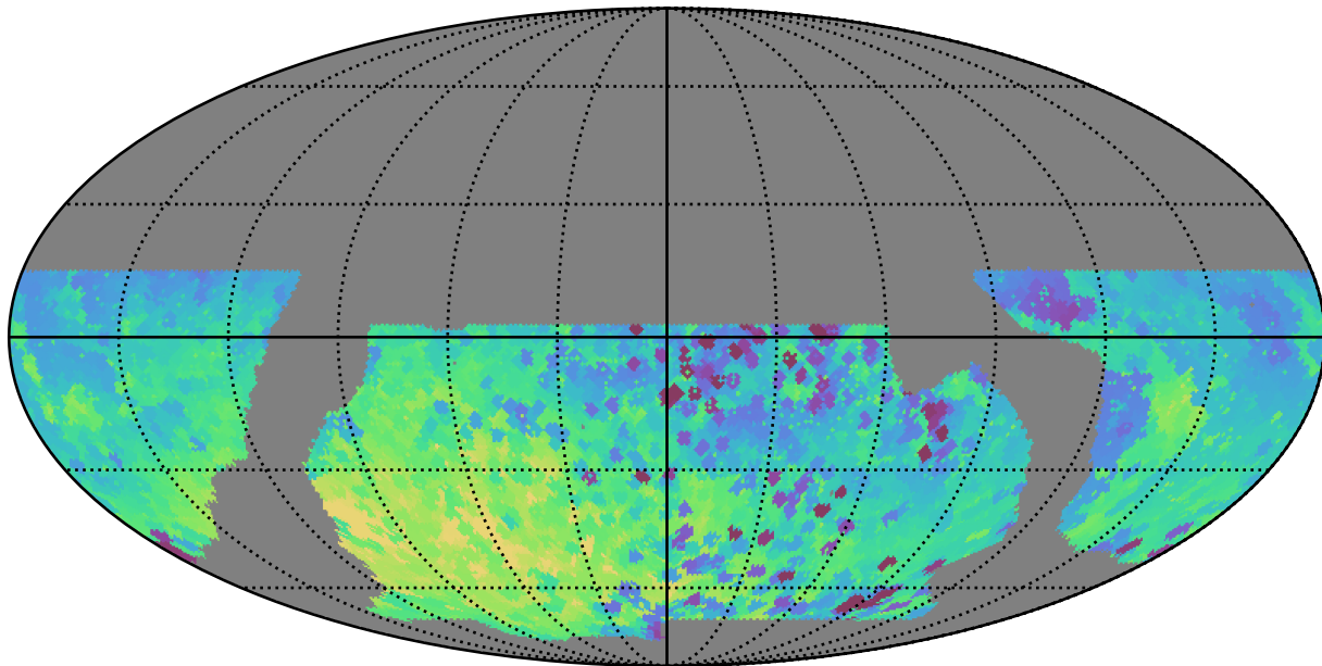
baseline_v2.0_10yrs WFD z band: Min skyBrightness
