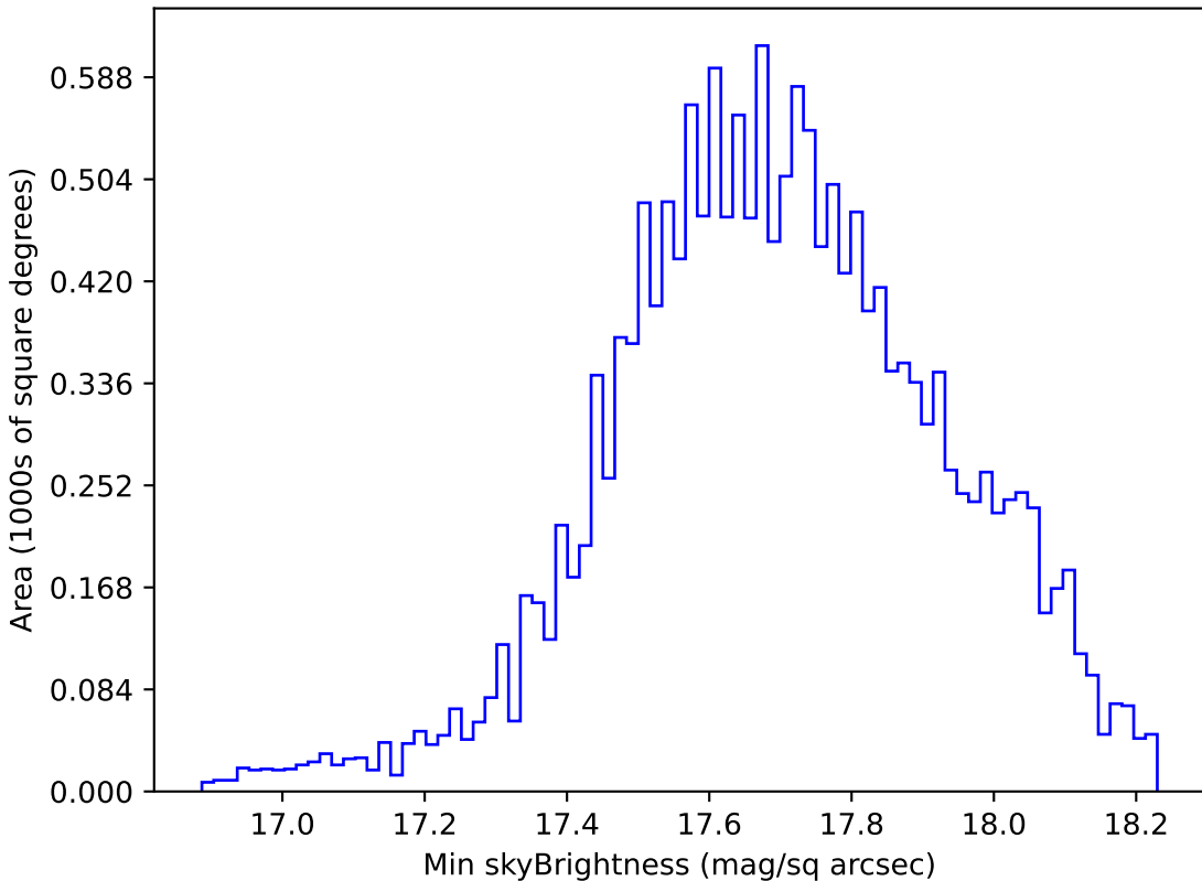
baseline_v2.0_10yrs WFD z band: Min skyBrightness
