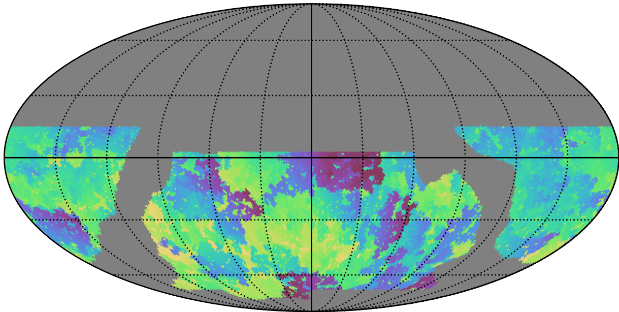
baseline_v2.0_10yrs WFD u band: Min skyBrightness
