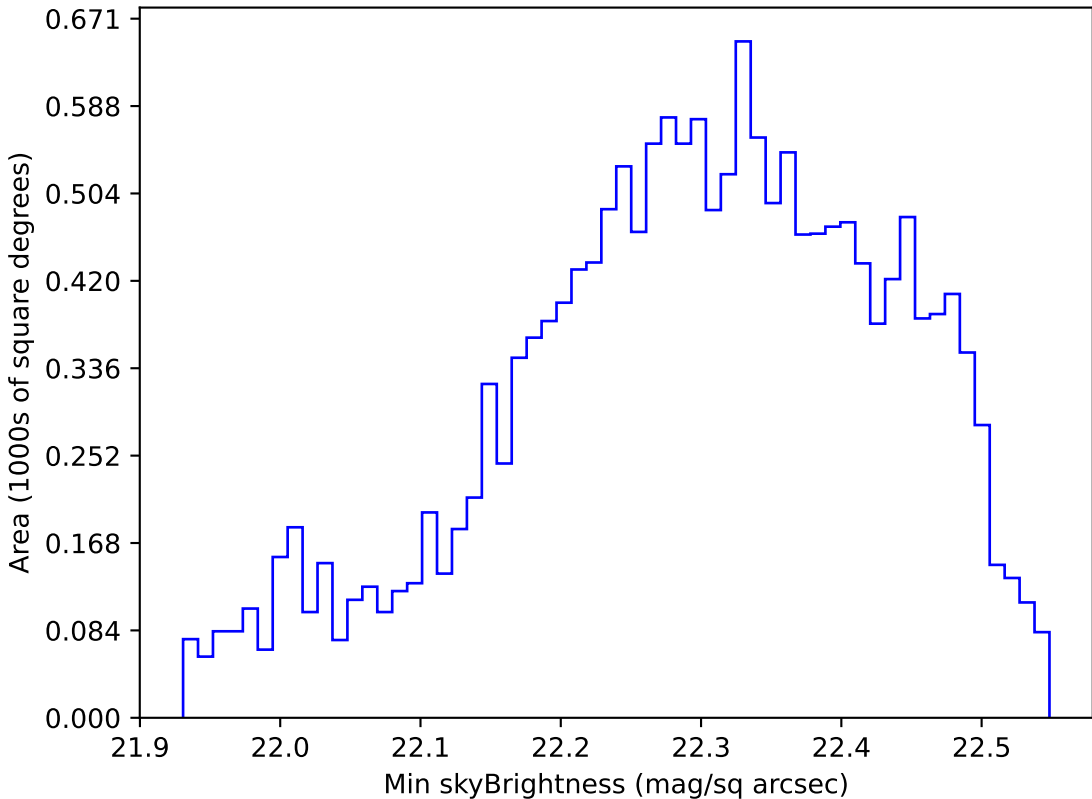
baseline_v2.0_10yrs WFD u band: Min skyBrightness
