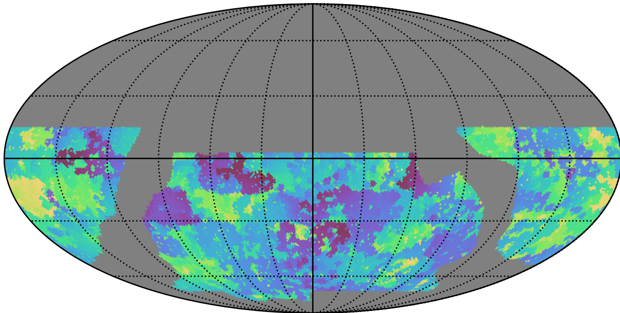
baseline_v2.0_10yrs WFD r band: Min skyBrightness
