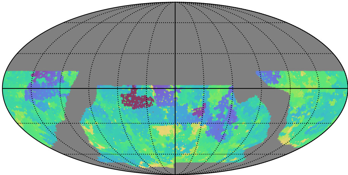
baseline_v2.0_10yrs WFD g band: Min skyBrightness
