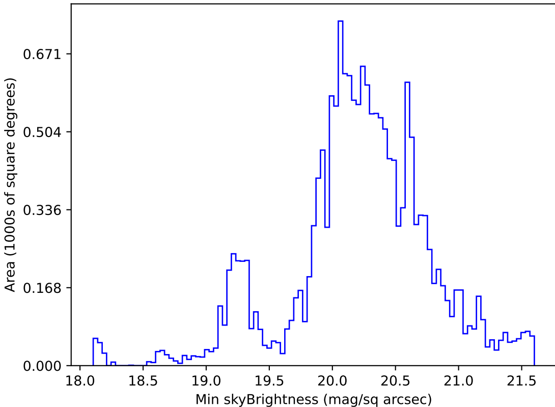
baseline_v2.0_10yrs WFD g band: Min skyBrightness
