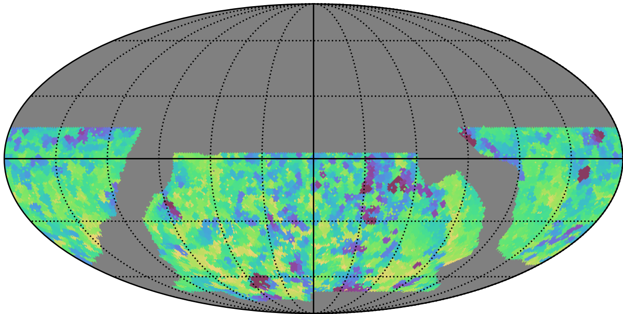
baseline_v2.0_10yrs WFD all bands: Min skyBrightness
