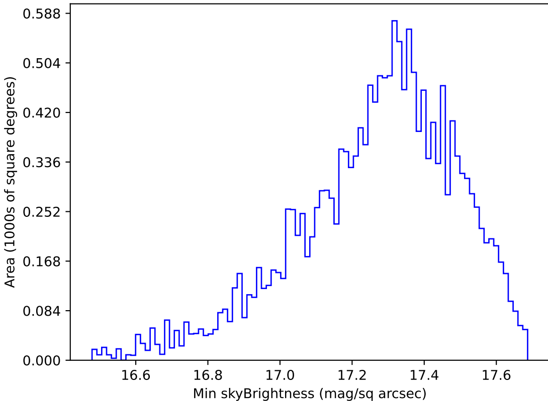
baseline_v2.0_10yrs WFD all bands: Min skyBrightness
