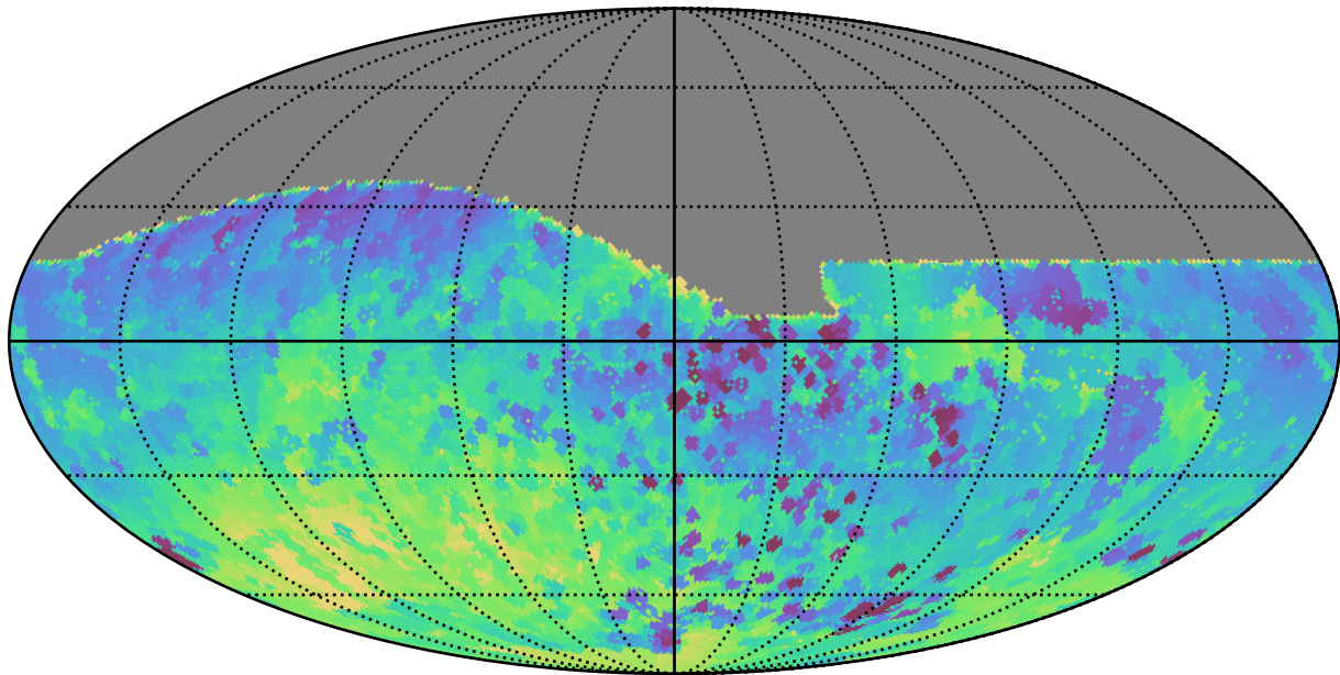
baseline_v2.0_10yrs All sky z band: Min skyBrightness
