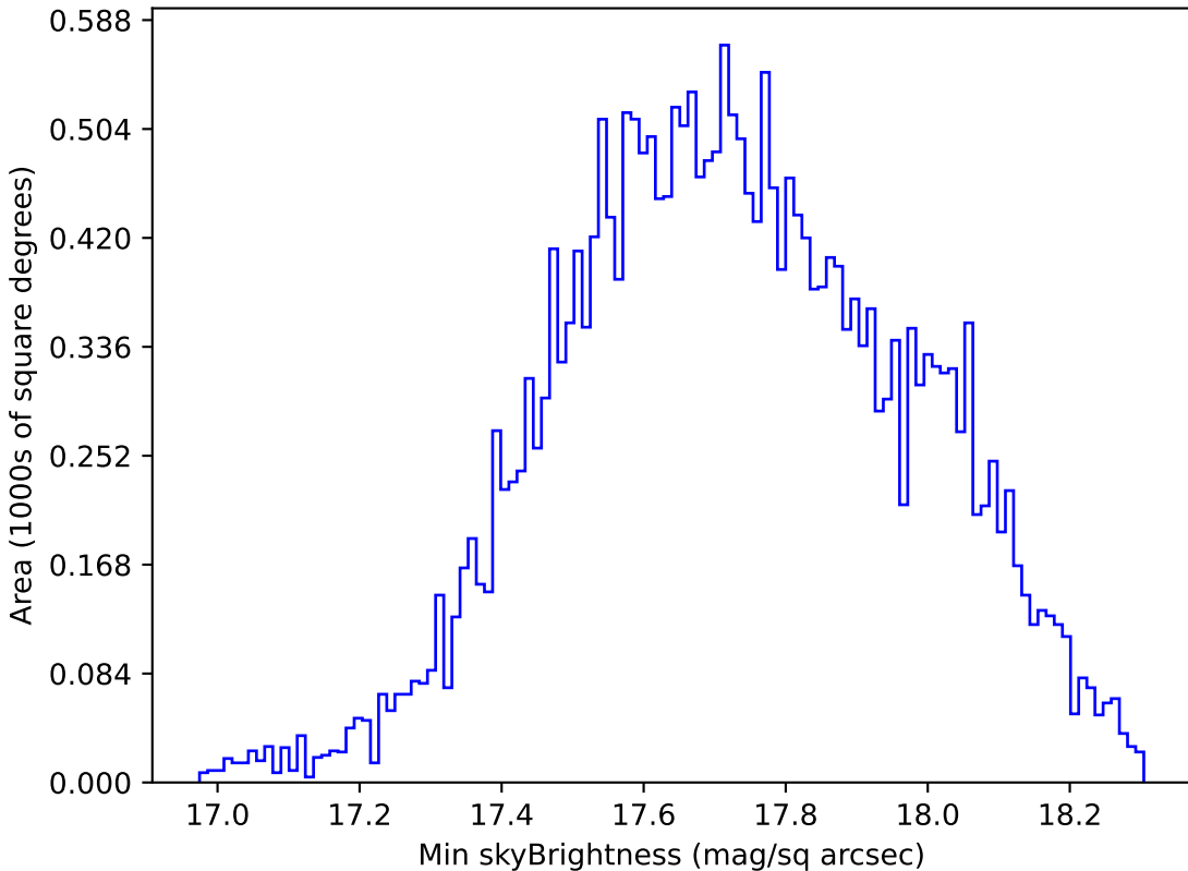
baseline_v2.0_10yrs All sky z band: Min skyBrightness
