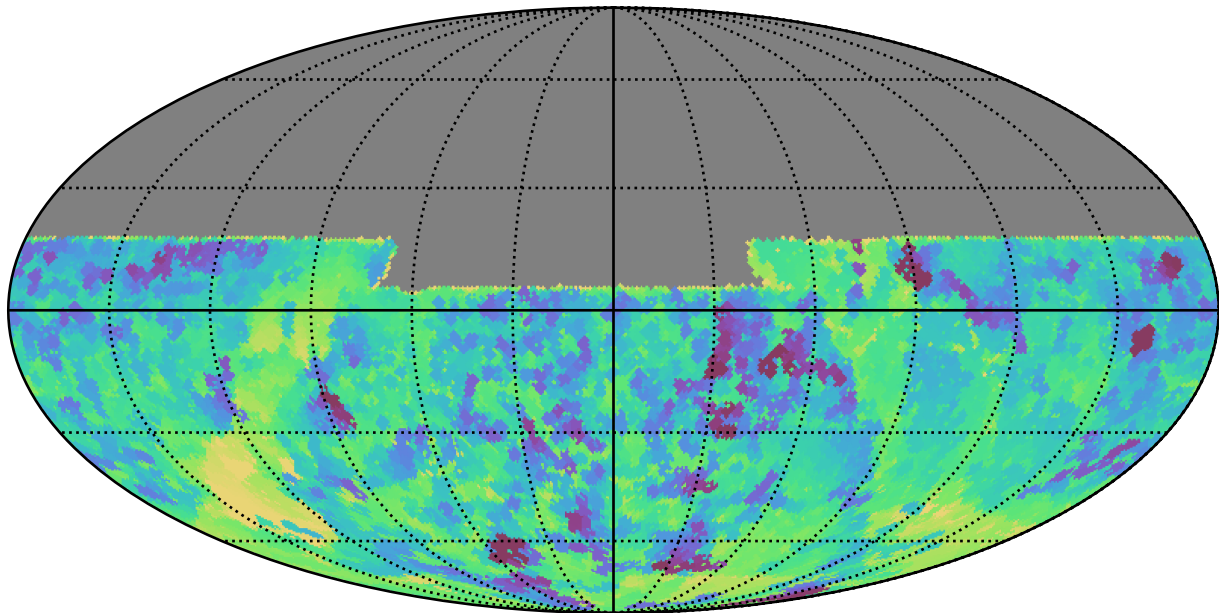
baseline_v2.0_10yrs All sky y band: Min skyBrightness
