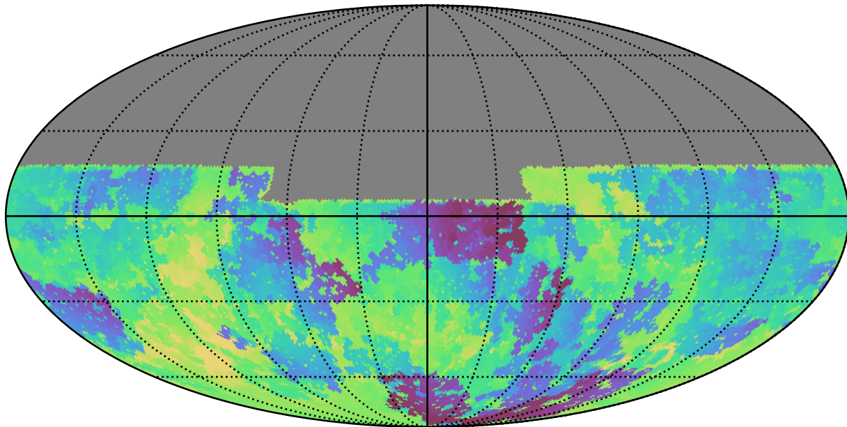
baseline_v2.0_10yrs All sky u band: Min skyBrightness
