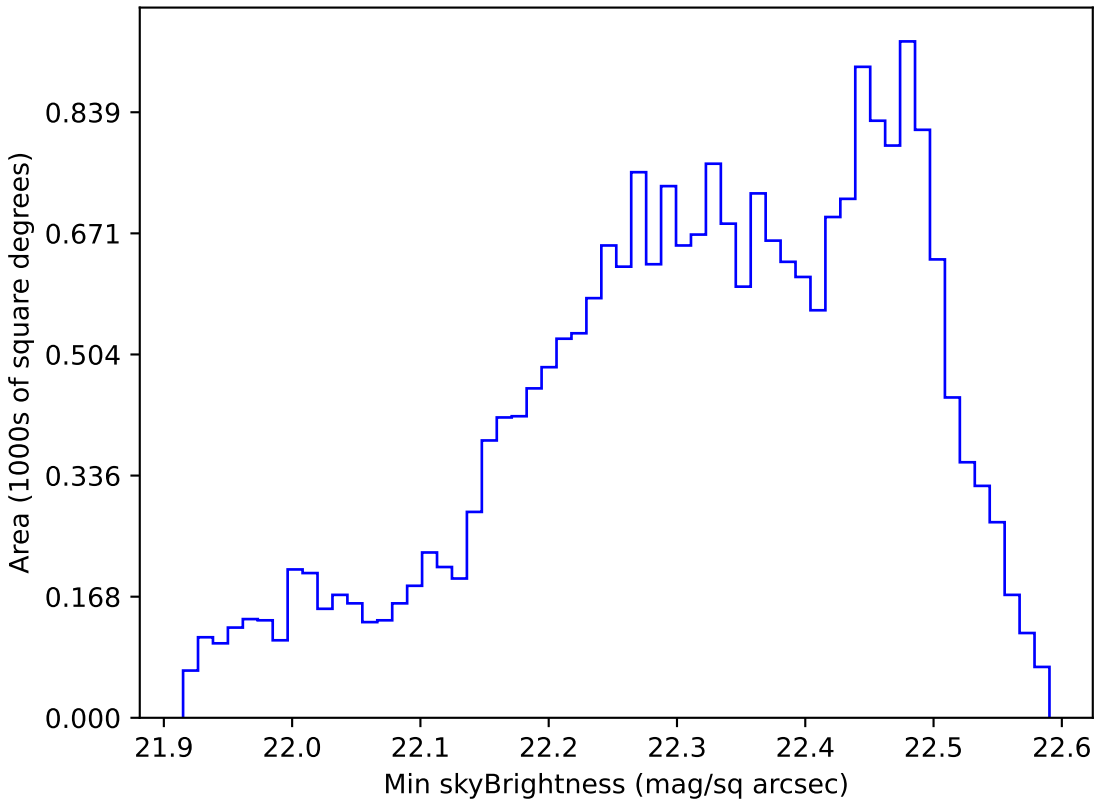
baseline_v2.0_10yrs All sky u band: Min skyBrightness
