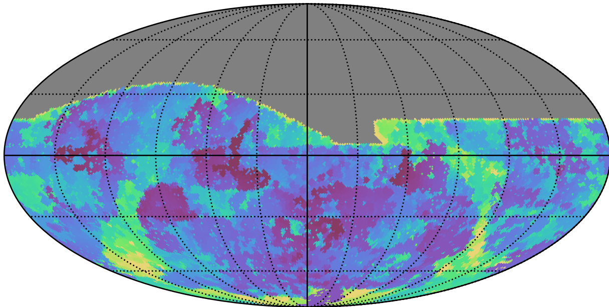
baseline_v2.0_10yrs All sky r band: Min skyBrightness
