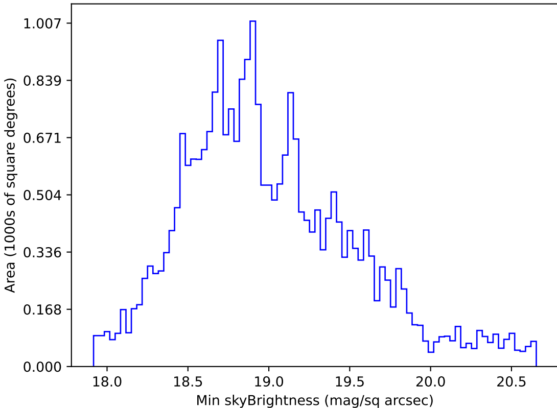
baseline_v2.0_10yrs All sky r band: Min skyBrightness
