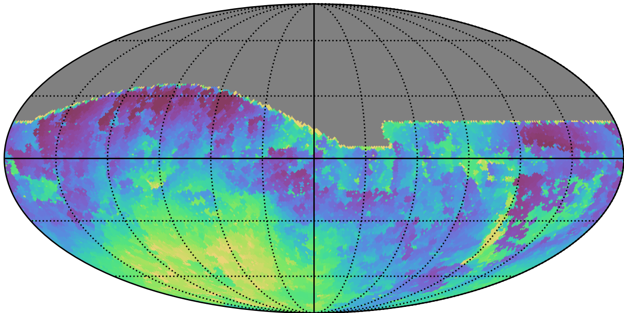
baseline_v2.0_10yrs All sky i band: Min skyBrightness
