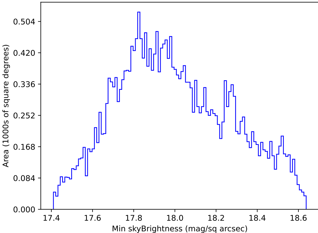
baseline_v2.0_10yrs All sky i band: Min skyBrightness
