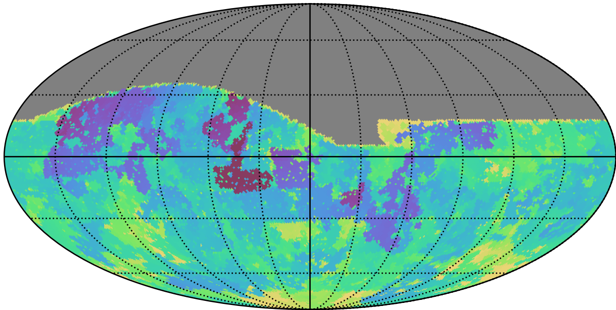
baseline_v2.0_10yrs All sky g band: Min skyBrightness
