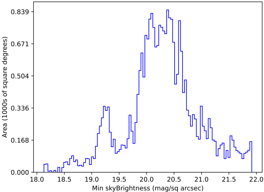
baseline_v2.0_10yrs All sky g band: Min skyBrightness
