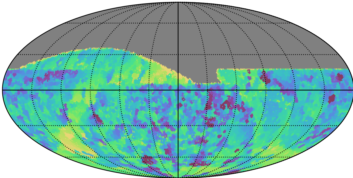
baseline_v2.0_10yrs All sky all bands: Min skyBrightness
