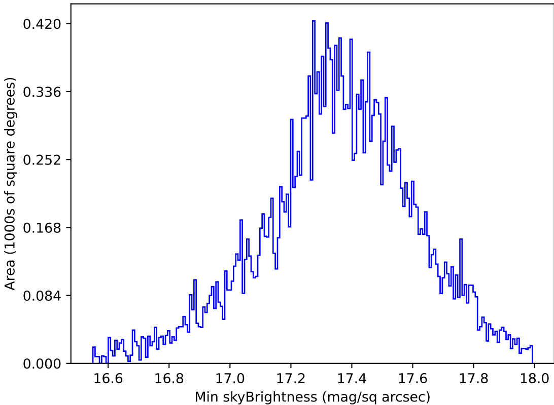
baseline_v2.0_10yrs All sky all bands: Min skyBrightness
