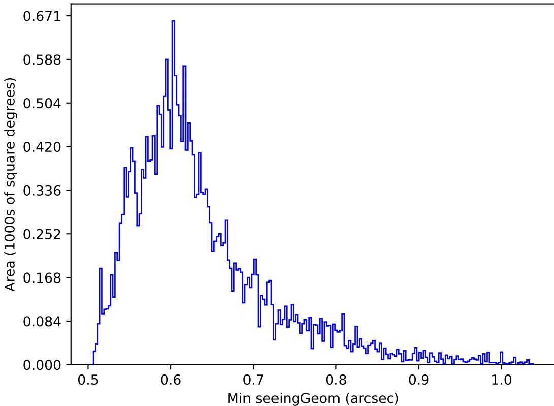
baseline_v2.0_10yrs Yr 1 z band: Min seeingGeom
