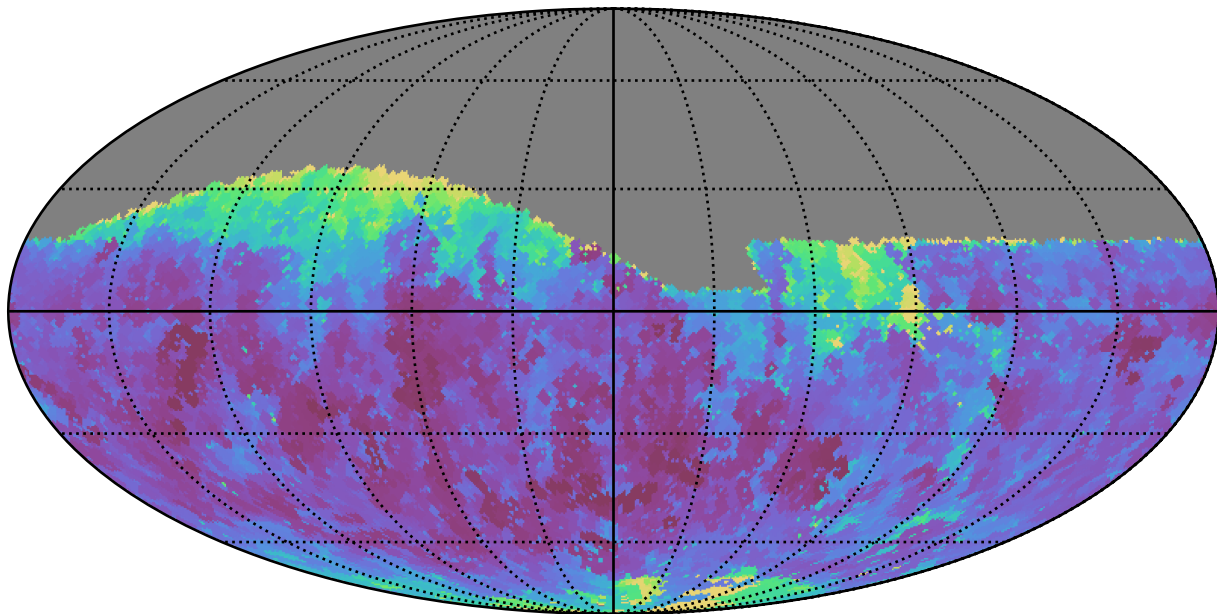
baseline_v2.0_10yrs Yr 1 r band: Min seeingGeom
