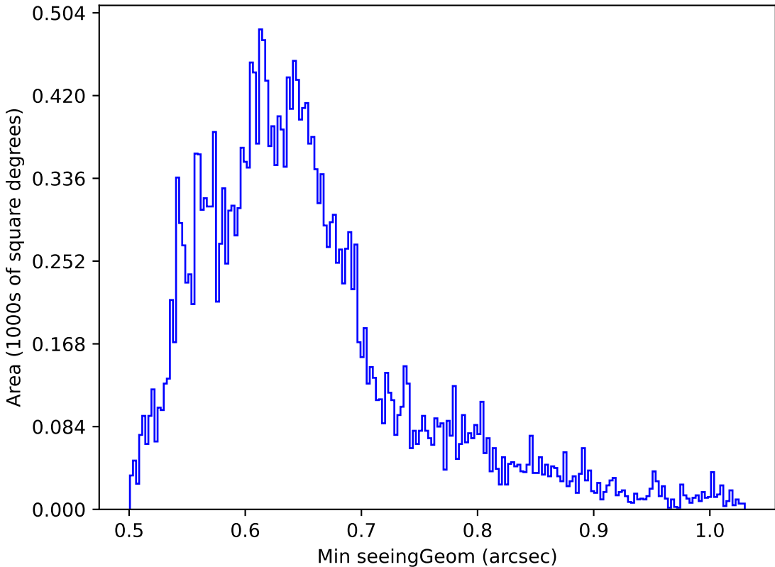
baseline_v2.0_10yrs Yr 1 r band: Min seeingGeom
