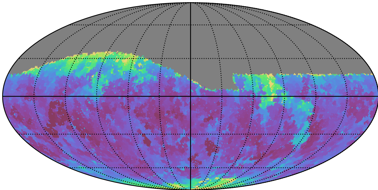
baseline_v2.0_10yrs Yr 1 i band: Min seeingGeom
