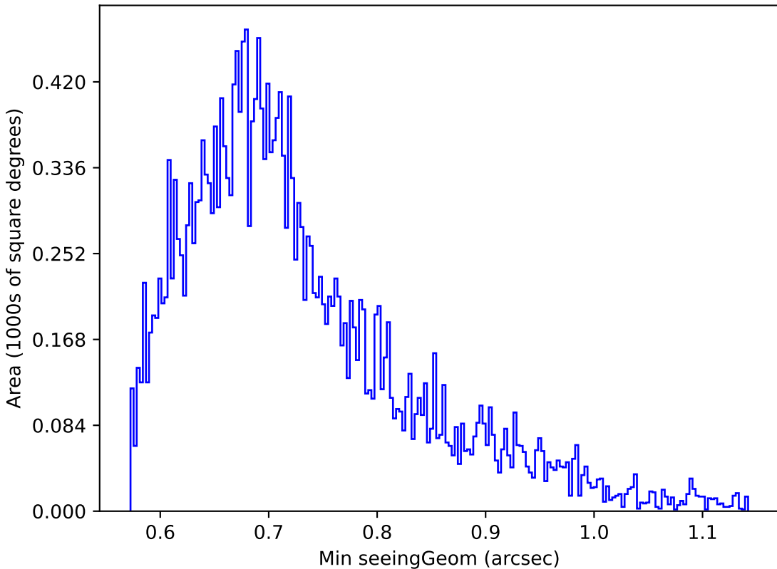
baseline_v2.0_10yrs Yr 1 g band: Min seeingGeom
