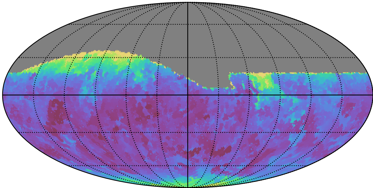
baseline_v2.0_10yrs Yr 1 all bands: Min seeingGeom
