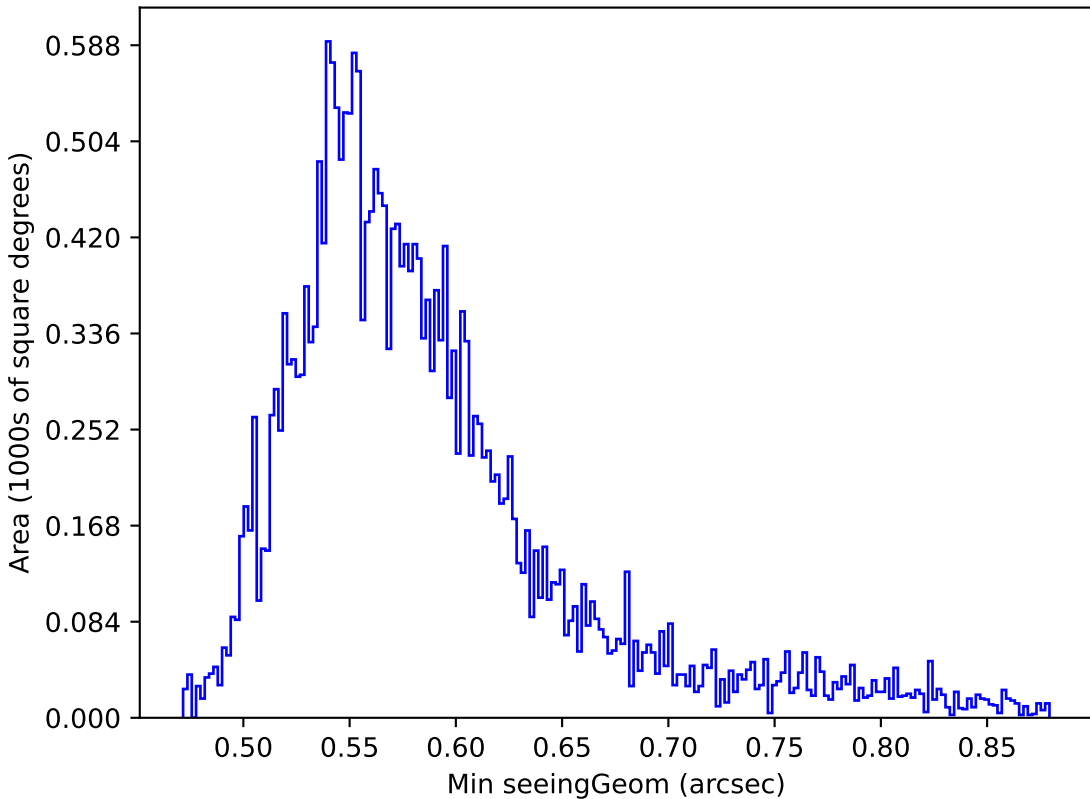
baseline_v2.0_10yrs Yr 1 all bands: Min seeingGeom
