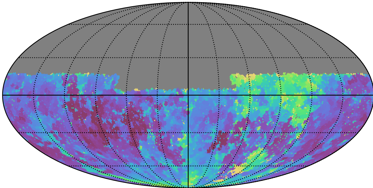
baseline_v2.0_10yrs Yr 1 u band: Min seeingEff
