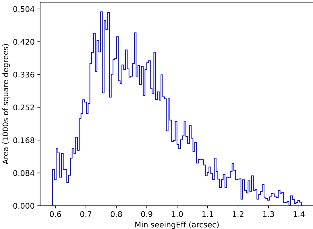
baseline_v2.0_10yrs Yr 1 u band: Min seeingEff
