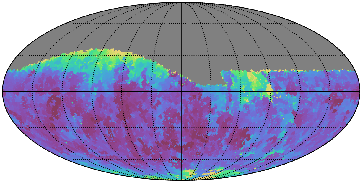
baseline_v2.0_10yrs Yr 1 r band: Min seeingEff
